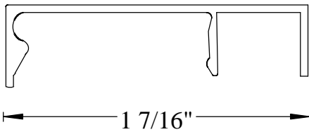
Full Face Perimeter Trim (TFF1)
